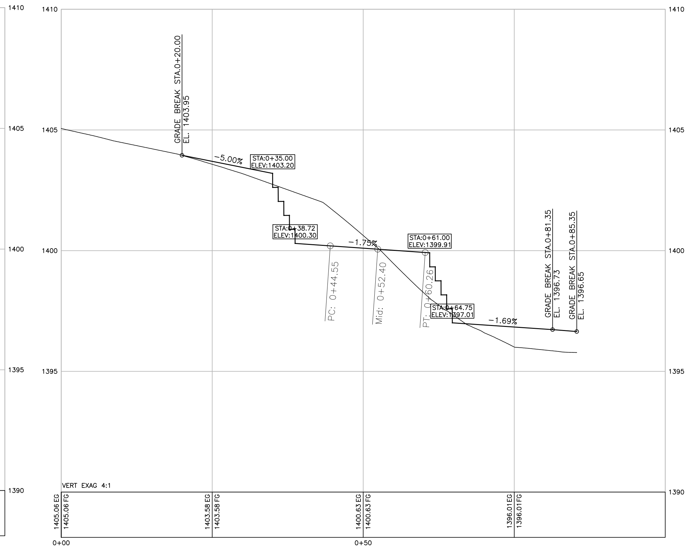
Profile of sidewalk extension and stair
